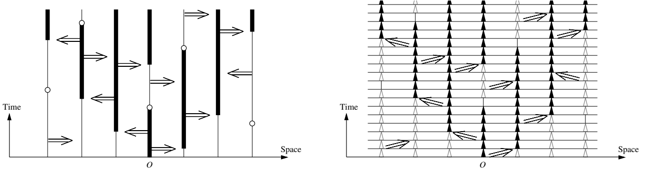
Figure 1: Graphical representation of the contact process and the discretized contact process.
