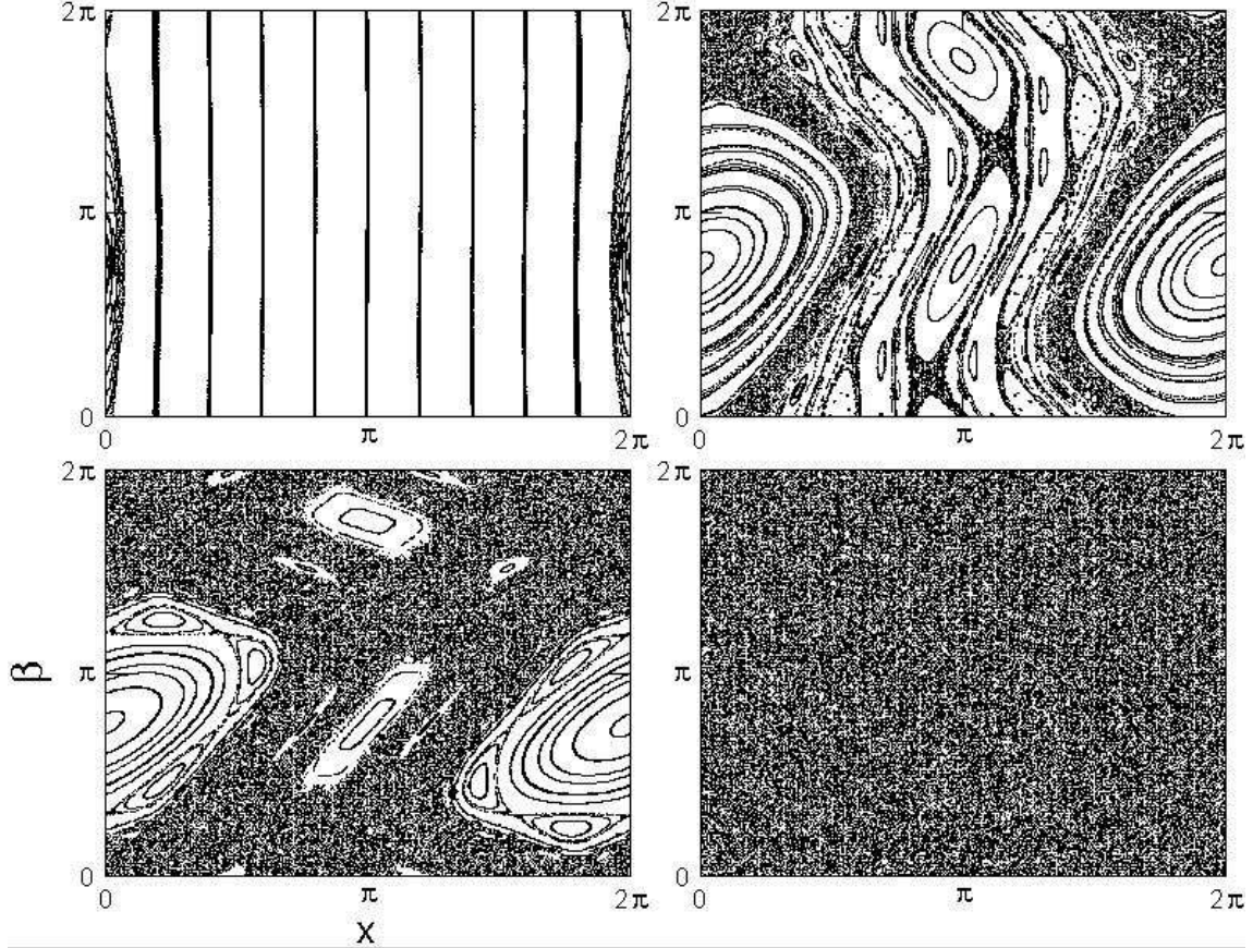
Figure 1: Poincaré sections for the map (19). Here A = 1 and v = 0.01 (top left), v = 0.6 (top right), v = 1 . (bottom left), v = 5 . (bottom right)
