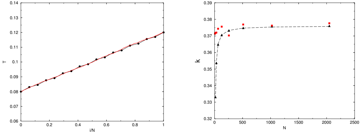
Figure 2: Results of simulations for A = 1 . Left: temperature profile with two heat baths for N = 16 (circles) and N = 2048 (full line). Right: Heat conductivity versus the chain length N obtained through non equilibrium simulations (squares) and GK formula (triangles). The continuous line represents the best fit with a function k_\infty + a/N .
