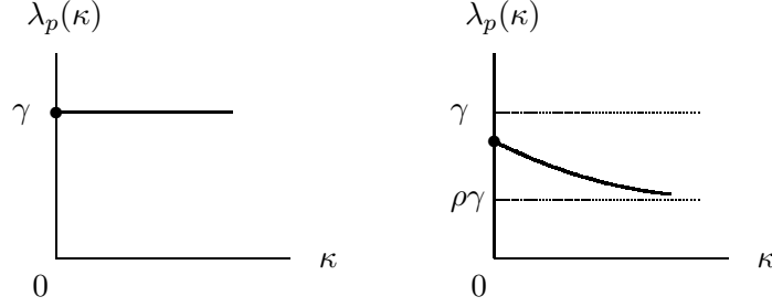
Figure 2: Qualitative picture of \kappa \mapsto \lambda_p(\kappa) for recurrent, respectively, transient random walk.
