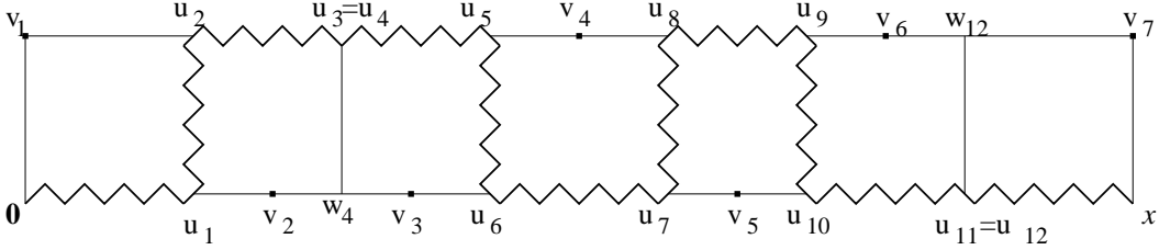
Figure 19: An example of the Feynman diagrams arising from the lace expansion. A jagged lines from u_{i-1} to u_i represents the quantity h_{m_i}(u_i - u_{i-1}) (derived from the backbone from 0 to x ). A straight line between two vertices u and v represents the quantity \rho(v - u) (derived from intersections of branches emanating from the backbone).
