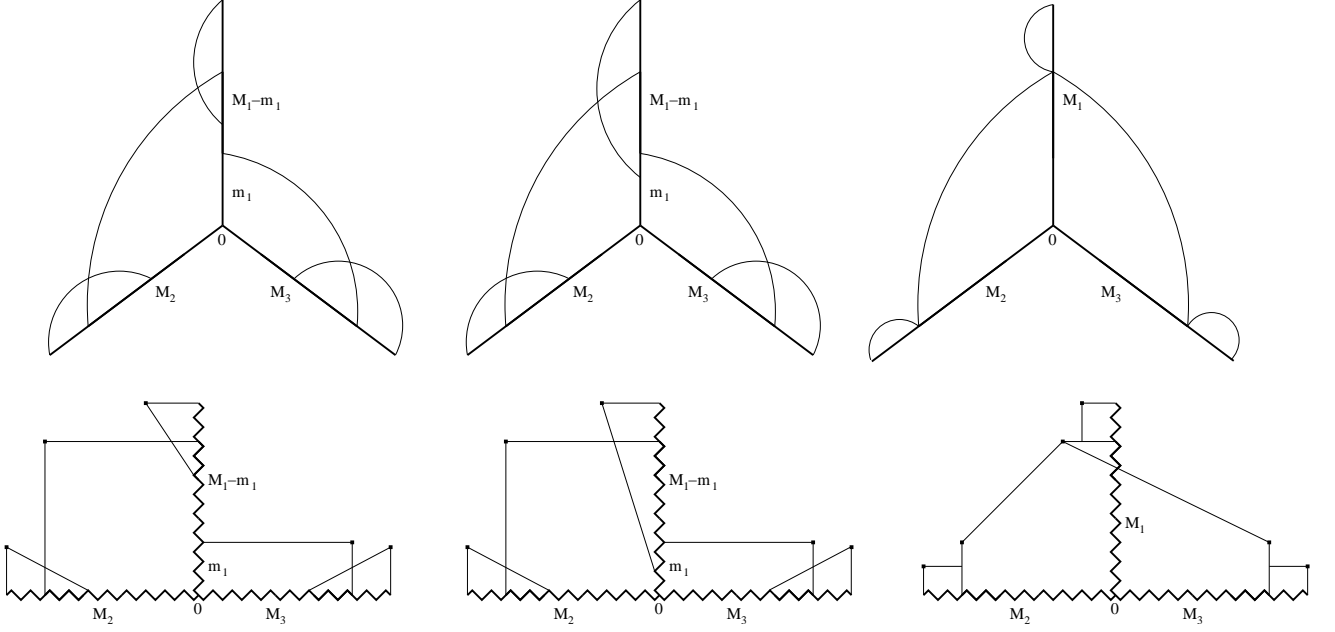
Figure 21: Three examples of acyclic laces with 2 bonds covering the branch point and more than two bonds in total and their diagrams (only one of the two topologically distinct possible diagrams for the third lace is shown).
