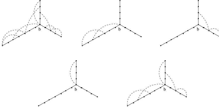
Figure 8: An illustration of the construction of a lace from a connected graph. The first figure shows a connected graph \Gamma on a star \mathcal{S}_{(n_1, n_2, n_3)}^3 . The intermediate figures show each of the \mathbf{L}_\Gamma(e) for e \in F_b , while the last figure shows the lace \mathbf{L}_\Gamma .
