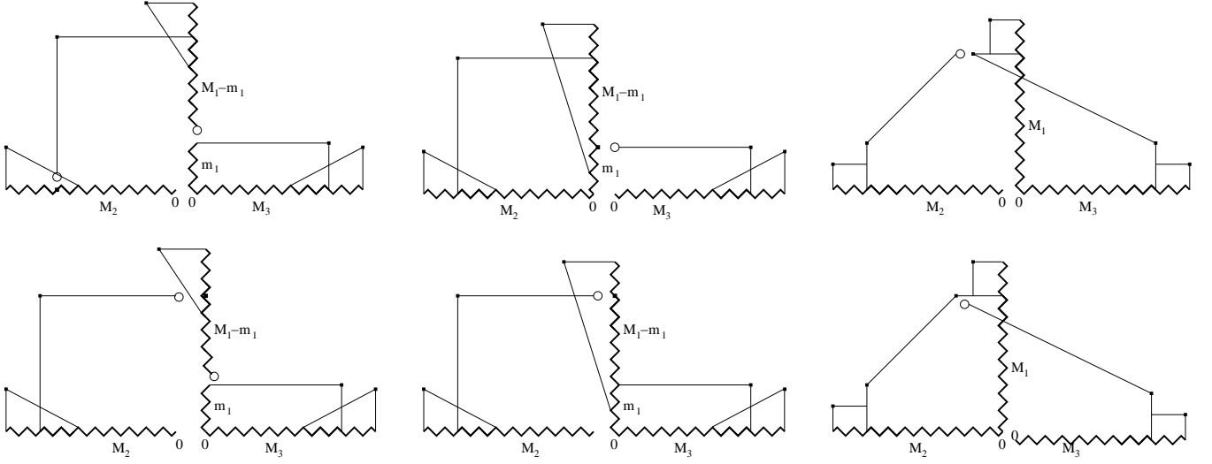
Figure 22: The first (resp. second, third) column shows the decompositions of the first (resp. second third) diagram of Figure 21. Apart from the second column, these are the same as the decompositions in Figure 20.
