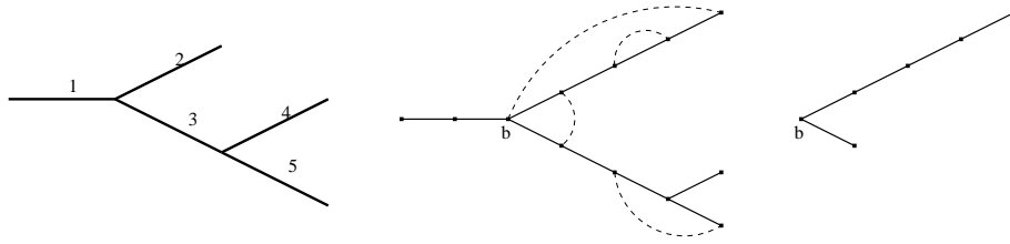
Figure 5: A shape \alpha \in \Sigma_r for r = 4 with fixed branch labellings, followed by a graph \Gamma on \mathcal{N}(\alpha, (2, 4, 3, 1, 1)) , and the subnetwork \mathcal{A}_b(\Gamma) .
