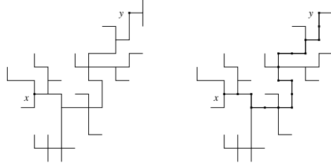
Figure 2: A nearest neighbour lattice tree in 2 dimensions. The backbone from x to y of length n = 17 is highlighted in the second figure.
