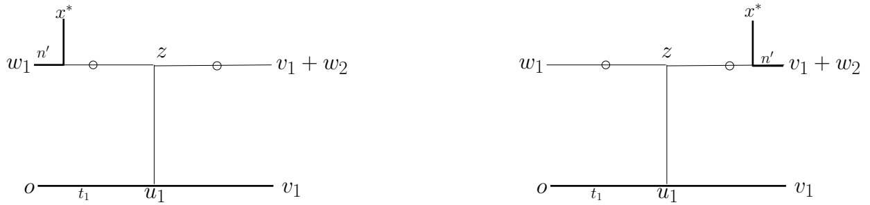
Figure 6: Two diagrams corresponding to a 2-edge lace with t_2 = 0 on a single branch, with an extra arm added at s_* = 0 or s_* = M respectively.
