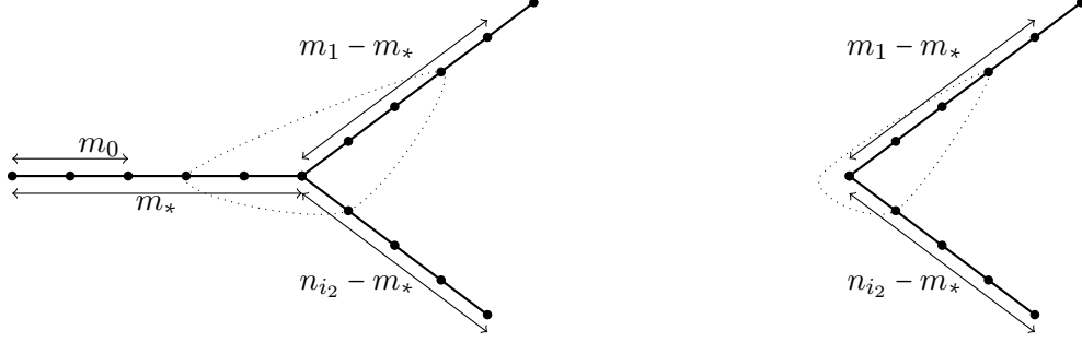
Figure 1: Two examples of star graphs \mathbf{S}_q^3 with branch lengths (q_0, q_1, q_2) = (m_*, n_1 - m_*, n_{i_2} - m_*) equal to (5, 5, 4) and (0, 5, 4) respectively. The dotted line represents where the lace expansion from the branch point has stopped, which defines m_1 - 1 \geq m_* , m_2 - 1 \geq m_* , and m_0 + 1 \leq m_* .
