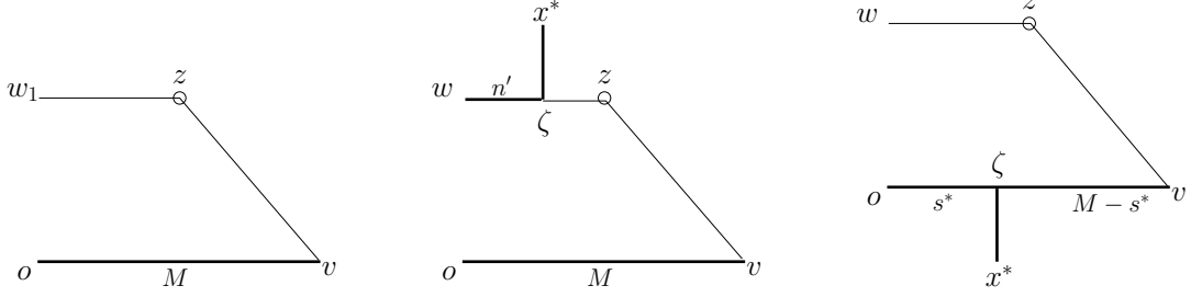
Figure 2: The diagram arising from a lace containing only one edge, and two of the diagrams arising from adding an extra arm; at s_* = 0 and 0 < s_* < M respectively. Dark lines correspond to h terms and light lines to \rho terms.
