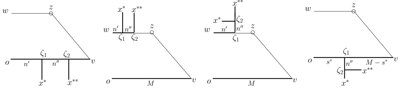
Figure 3: Some of the diagrams arising from a lace containing only one edge, with two extra arms added at s_* and s_{**} . From left to right the figures correspond to the situations where 0 < s_* < s_{**} < M , two cases of s_* = s_{**} = 0 , and 0 < s_* = s_{**} < M respectively.
