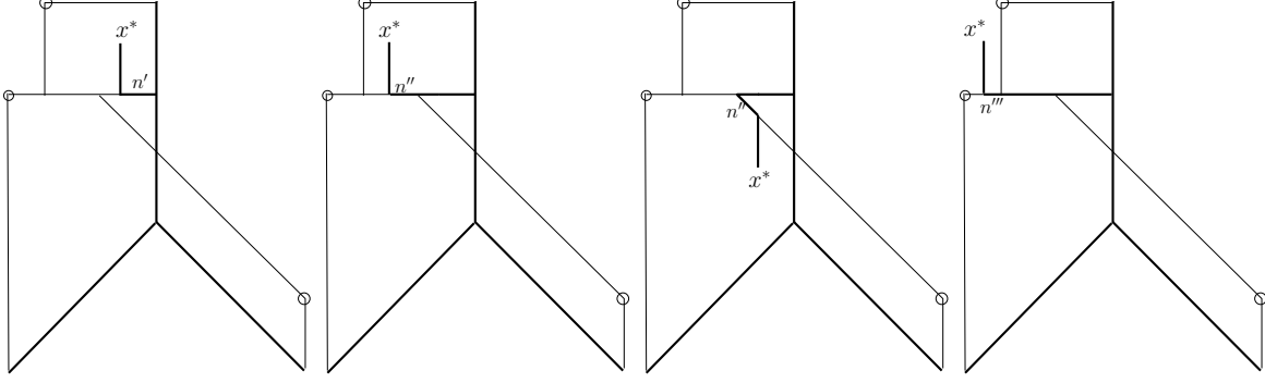
Figure 10: Some adjusted diagrams from adding an arm at the coincidence point of three endpoints of edges, for the diagram in Figure 9.
