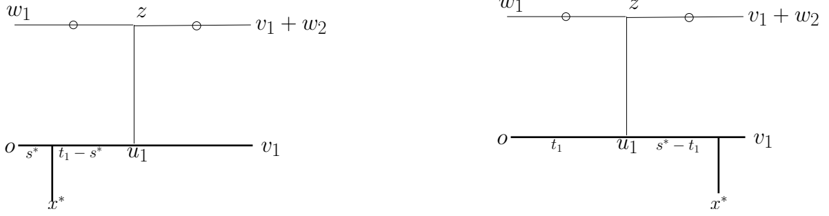
Figure 5: Two diagrams corresponding to a 2-edge lace (with t_2 = 0 ) on a single branch, with an extra arm added at s_* , where 0 < s_* < t_1 and t_1 < s_* < M respectively.
