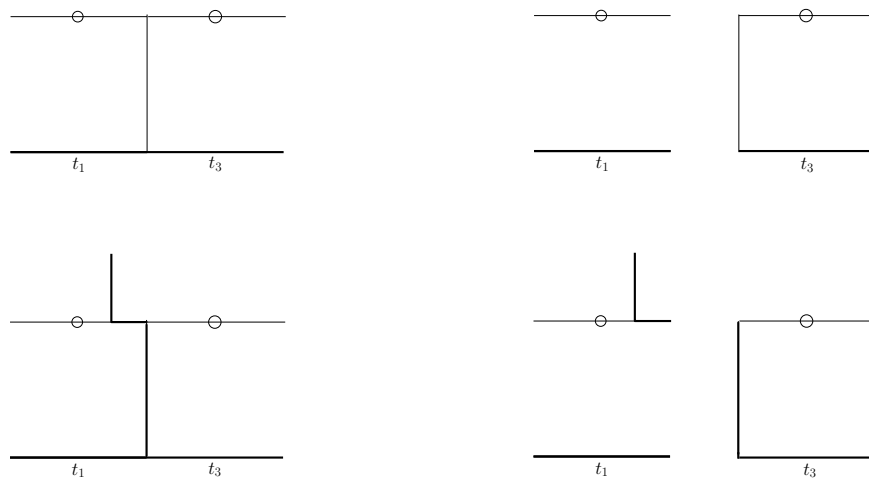
Figure 8: On the left are two diagrams (see the rightmost diagrams of Figures 4 and 7) corresponding to a 2-edge lace without and with an extra arm added. The same decomposition is used in each case. The decomposition when t_1 \geq M - t_1 appears on the right.
