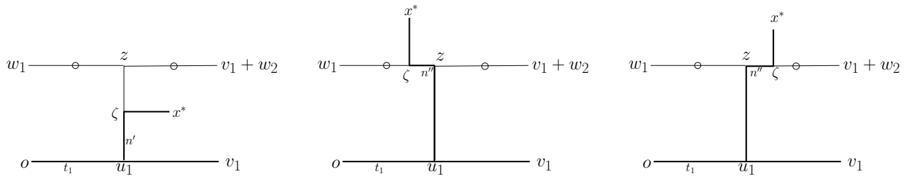
Figure 7: Three diagrams corresponding to a 2-edge lace with t_2 = 0 on a single branch, with an extra arm added at s_* = t_1 .
