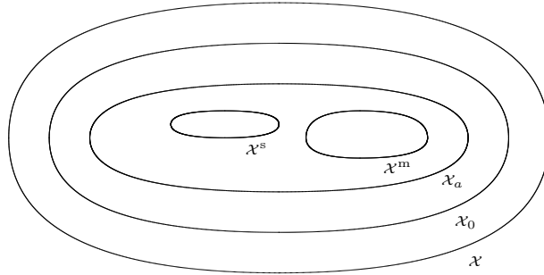
Fig. 2 Illustration of the structure of the sets \mathcal{X}_a 's (see definition (14)) with 0 < a < V^m .
