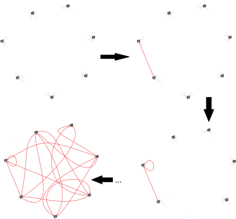
FIGURE 3. Illustration of the construction of \text{CM}_n . Three steps in the matching of stubs for n = 7 and degree sequence (5, 5, 4, 5, 5, 3, 5) .
