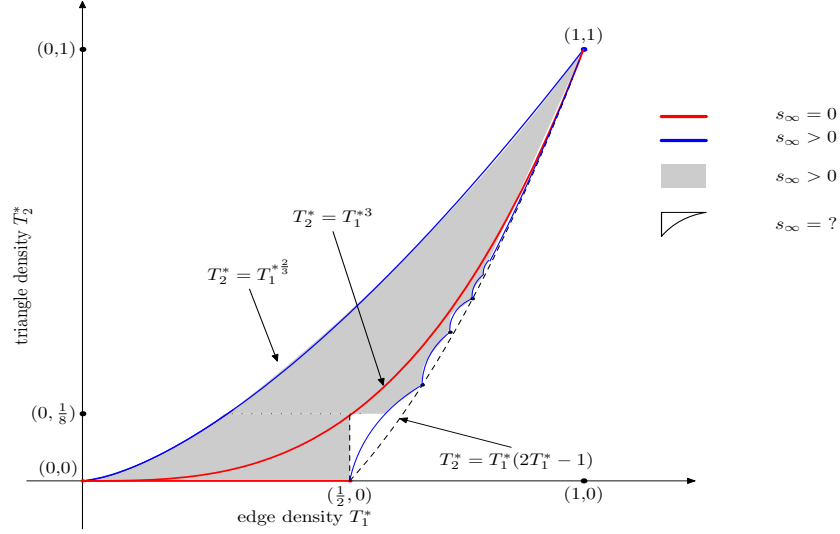
Figure 3: The admissible edge-triangle density region is the region on and between the blue curves (cf. Radin and Sadun [15]).
