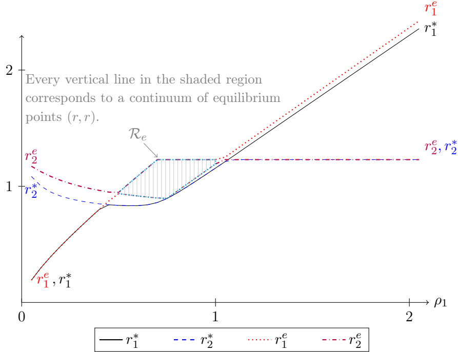
Figure 2: The optimal rates (r_1^*, r_2^*) and equilibrium rates (r_1^e, r_2^e) as a function of \rho_1 when all other parameters are fixed: K_1 = 3 , K_2 = 2 , k_1 = k_2 = 1 , p_1 = p_2 = 0.5 , \rho_2 = 0.7 , b_1 = b_2 = 0.08 , c_1 = c_2 = 0 , a_1 = a_2 = 0.1
